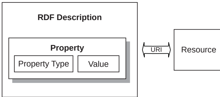
The RDF data model
